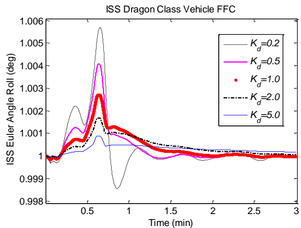
Figure 8 ISS Roll Angle for Various PD K_d Gains.
