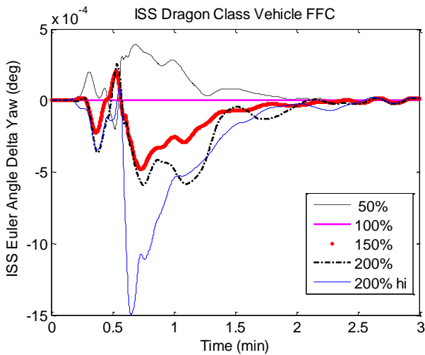
Figure 20 ISS Delta Yaw to Baseline Mass-PD Control.
